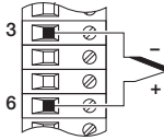
e – Thermocouple
