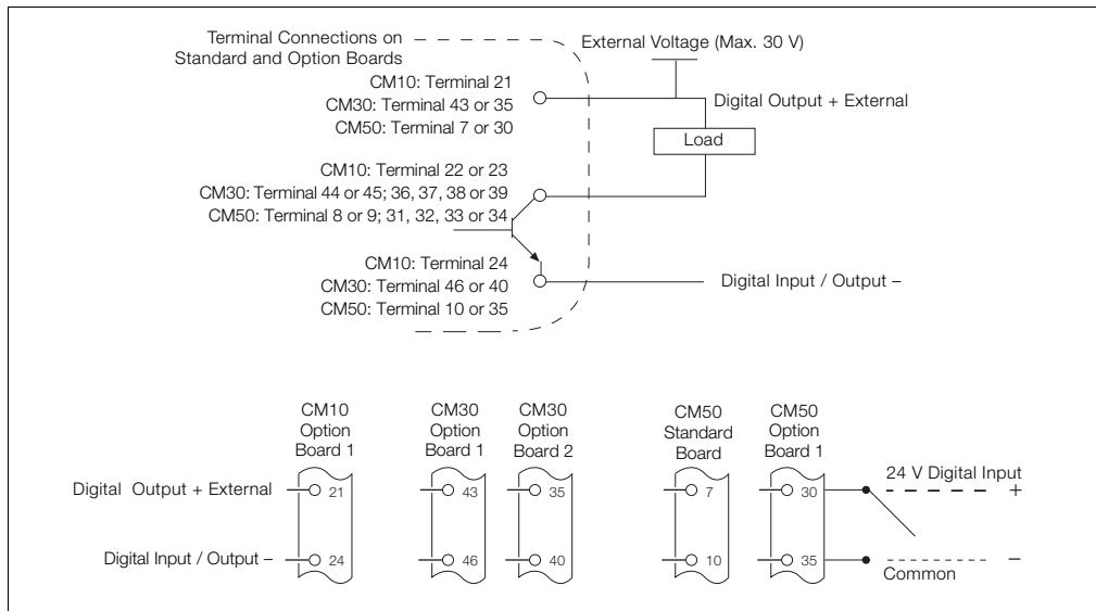
Fig. 4.13 Open Collector Digital Input / Output Connections
