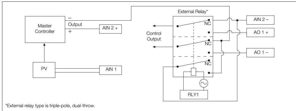
Fig. 8.4 Parallel Connection
