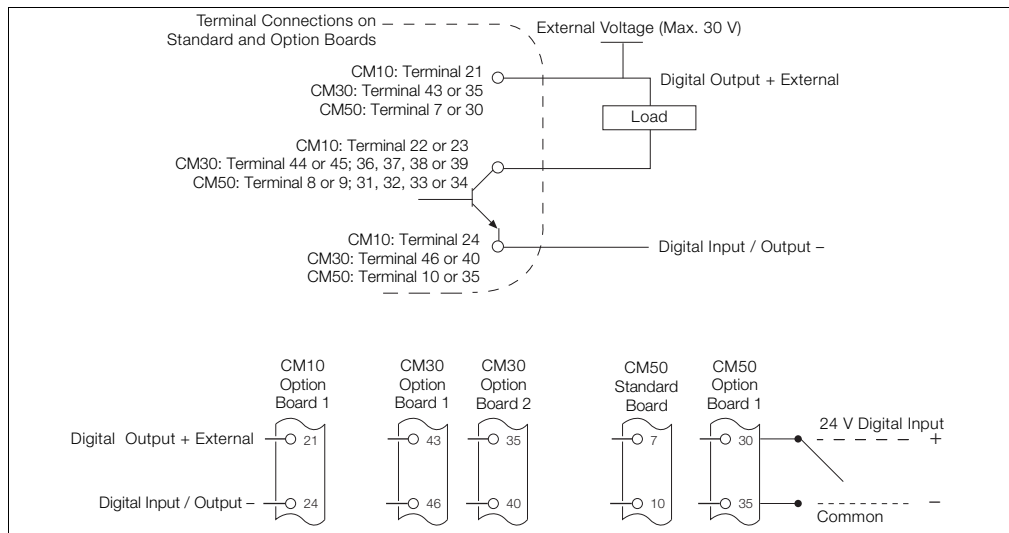
Fig. 4.13 Open Collector Digital Input / Output Connections
