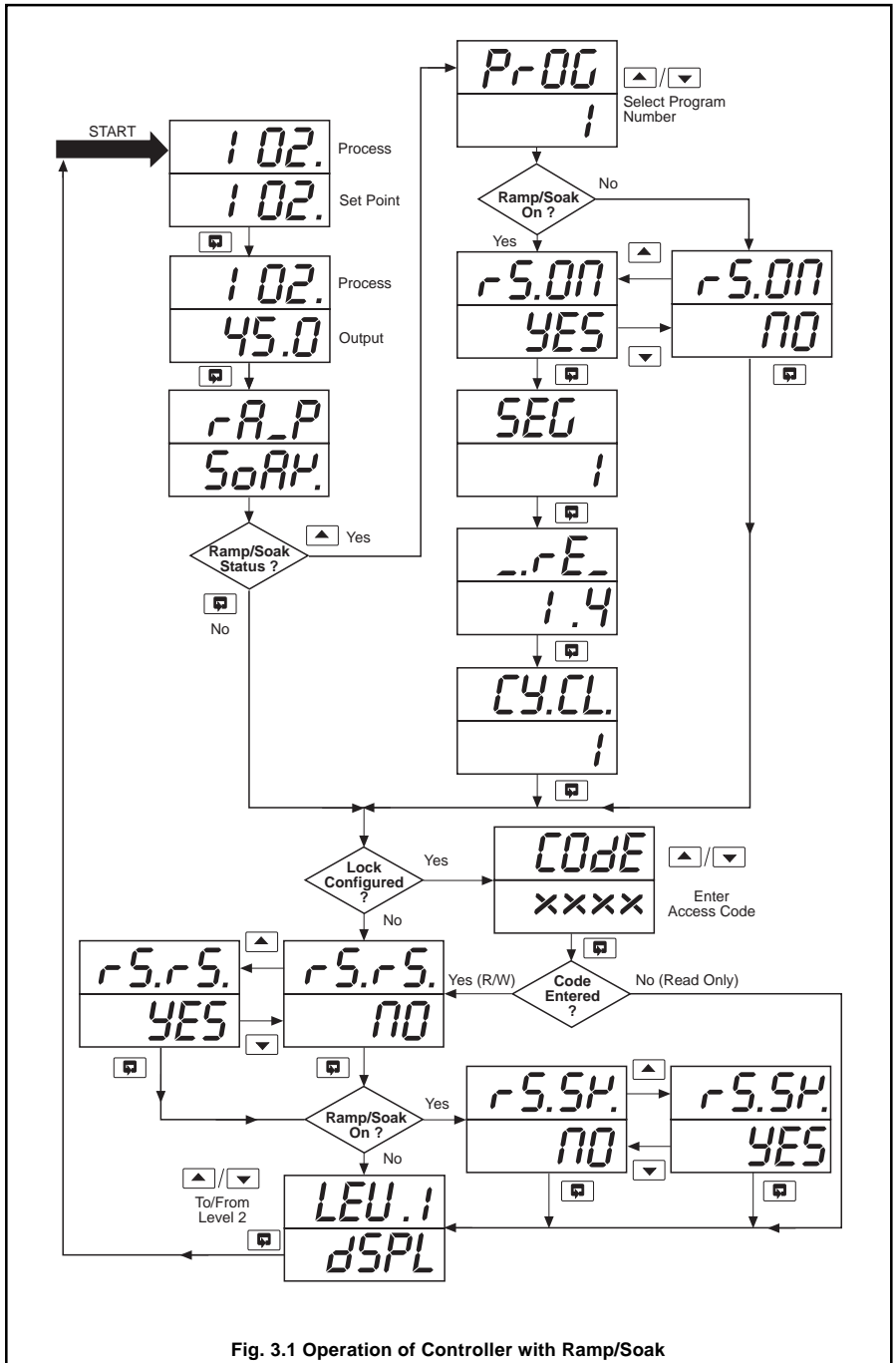
Fig. 3.1 Operation of Controller with Ramp/Soak
